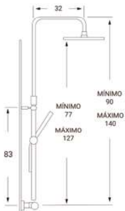
COLUMNA TERMOSTATICA EXTENSIBLE REDONDA BAÑERA MODELO TALIA THERMOSTATIC EXTENSIBLE COLUMN BATH/SHOWER
